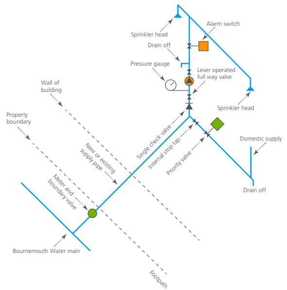
Fig 4 – Mains Fed Sprinkler Installation via a Single Metered Connection
