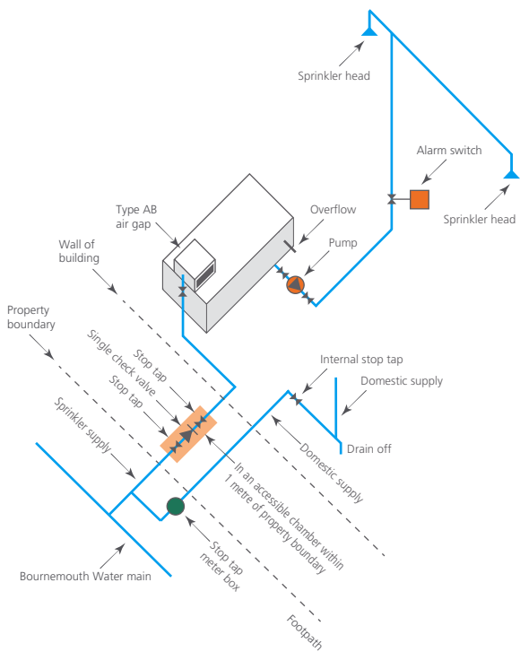
Fig 1 – Storage and Boosted Sprinkler Supply via Unmetered Branch Pipe
